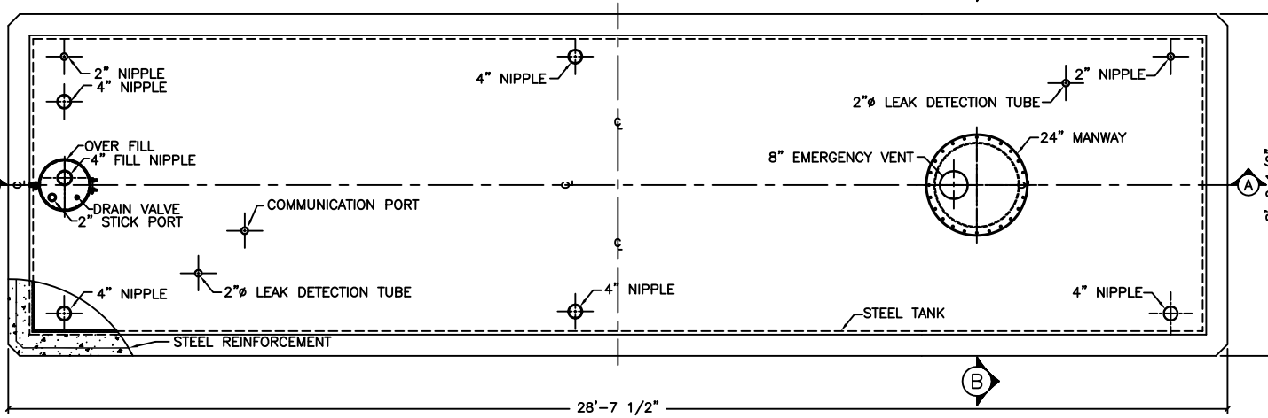
PLAN VIEW
