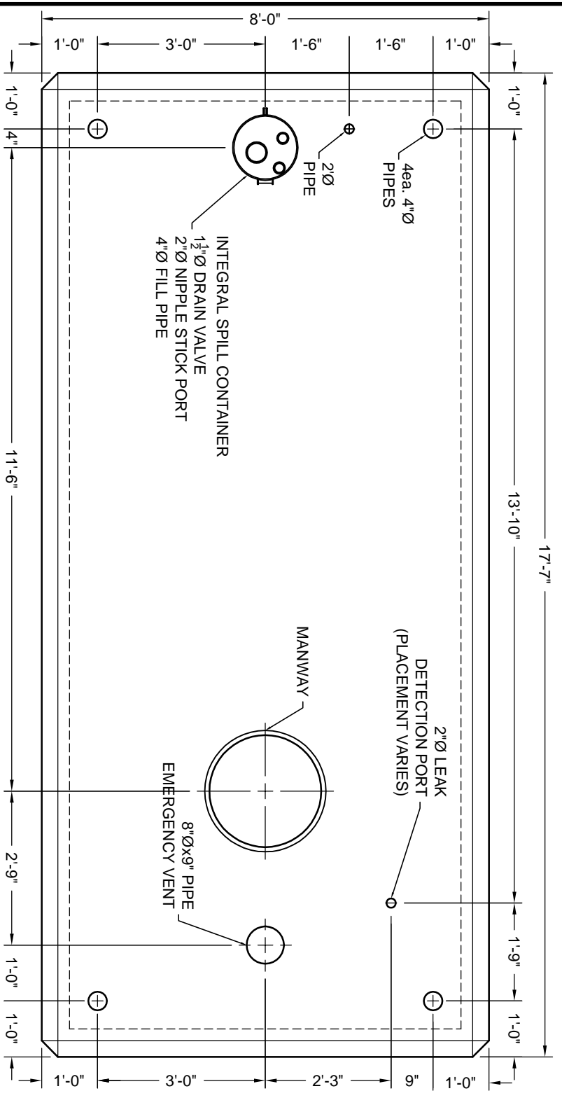
TYPICAL PLAN VIEW
